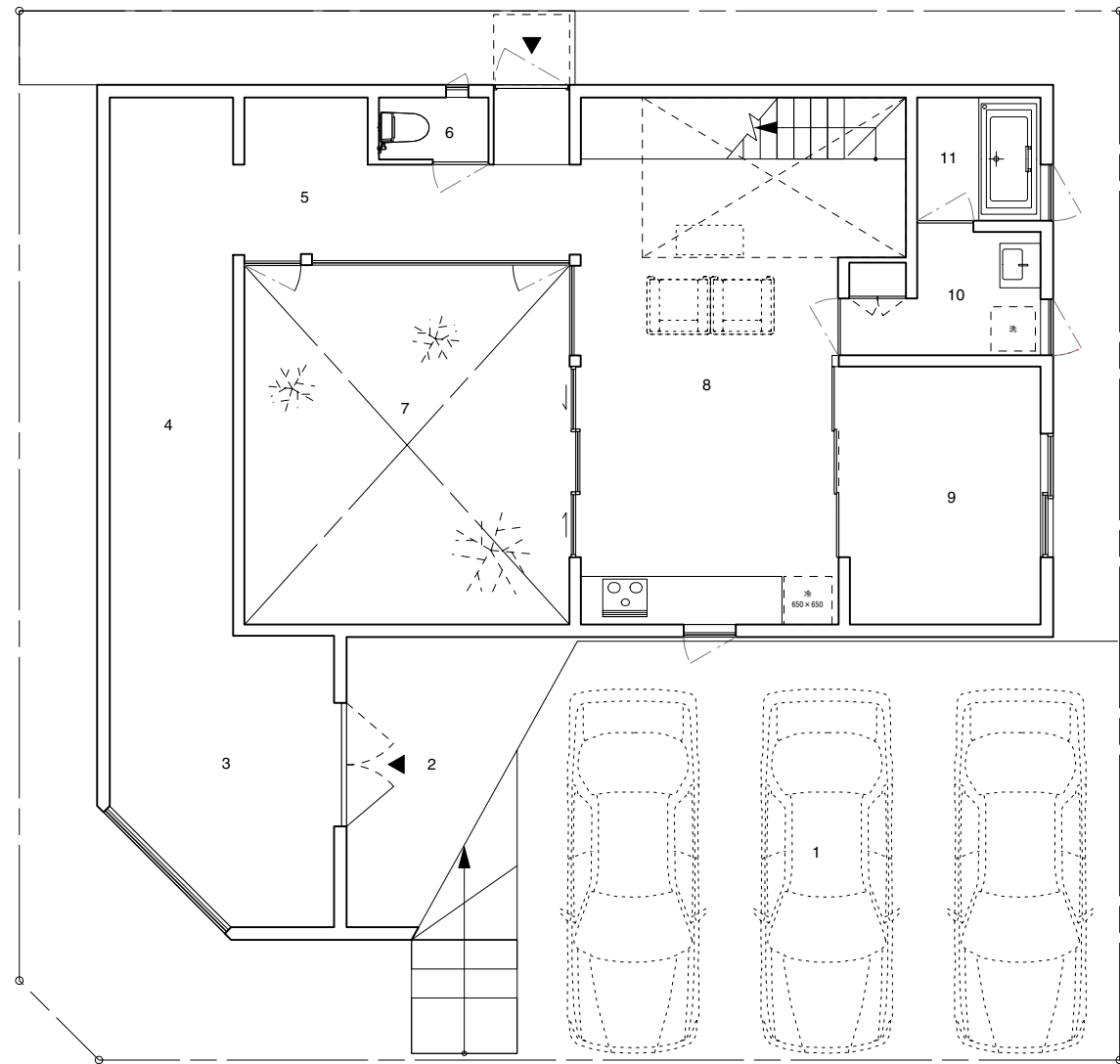
1F PLAN
